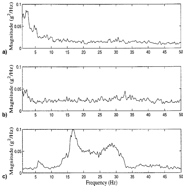
Fig. 2 PSD in g^2/Hz of right wing aileron accelerometer data in response to a) atmospheric turbulence, b) pilot commanded lateral stick raps, and c) wingtip excitation system.
