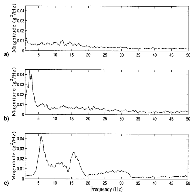
Fig. 1 PSD in g^2/Hz of left wing forward wingtip accelerometer data in response to a) atmospheric turbulence, b) pilot stick commanded lateral stick raps, and c) wingtip excitation system.
